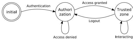
Fig. 1. Static authorization
