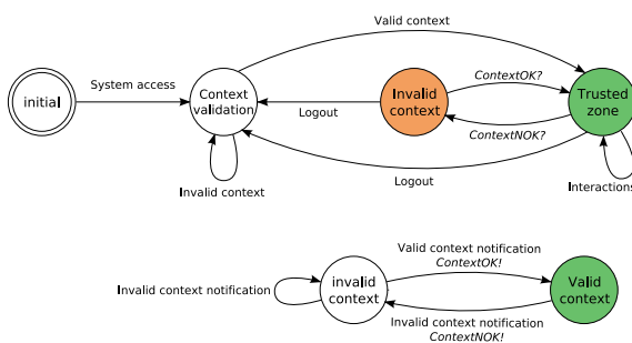
Fig. 3. Event-driven dynamic authorization
