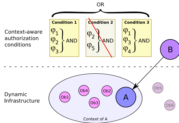
Fig. 6. Authorization conditions and based on observers availability
