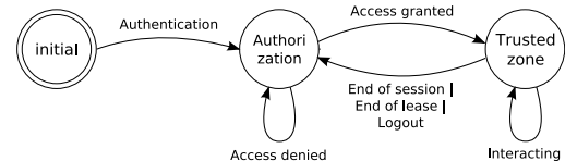
Fig. 2. Quasi-static authorization
