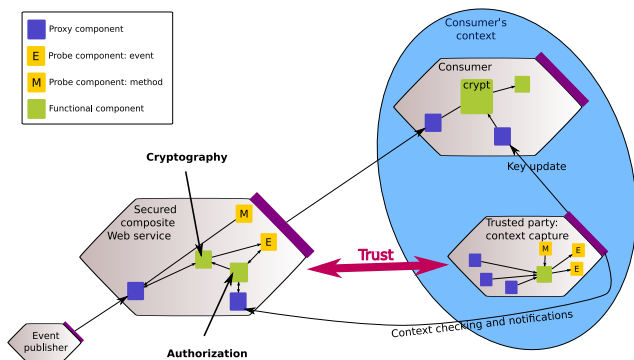
Fig. 8. Implementation using SLCA
